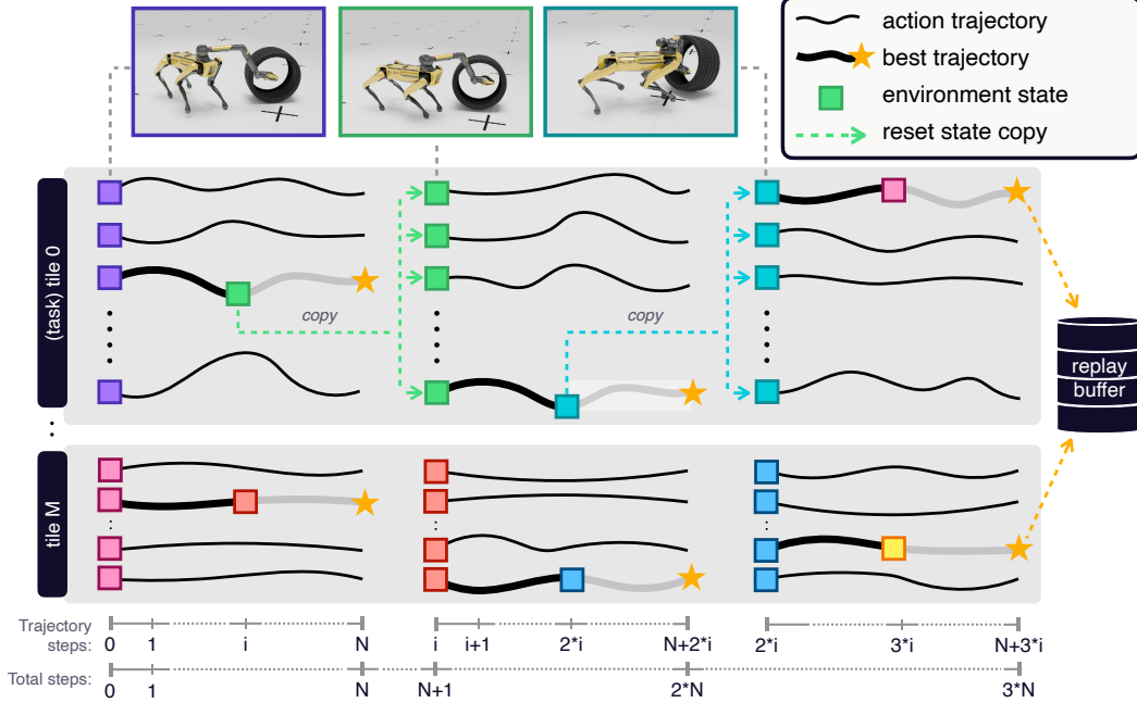
Figure 3: We scale our SMPC data collection by solving multiple SMPCs in parallel on the GPU using vectorized environments divided into tiles. Each tile broadcasts its initial task to all its environments upon reset, runs sampled actions, selects the best trajectories, and adds them to our expert buffer. Note the different x-axes scales for a task’s trajectory steps and total simulation steps.
